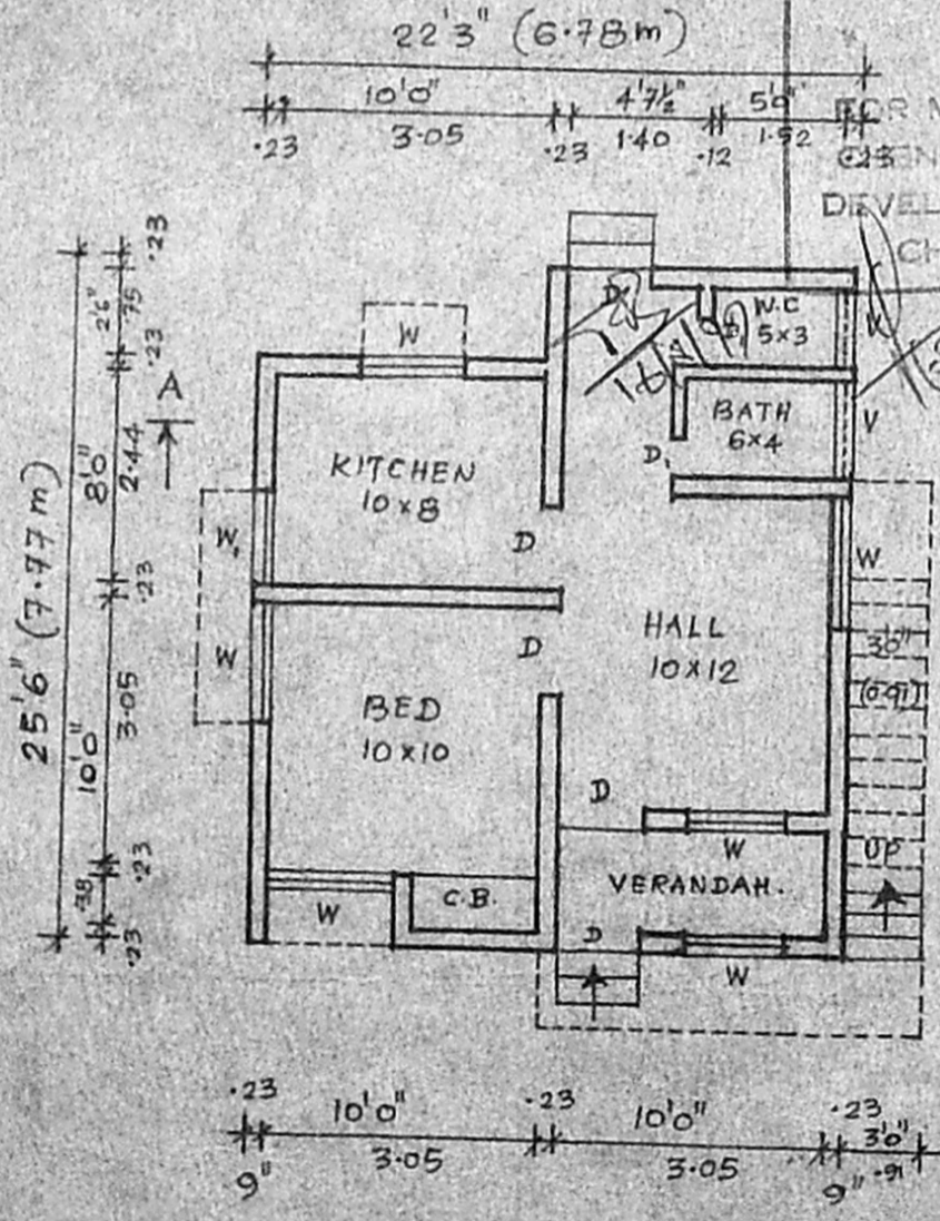
EX-GROUND FLOOR PLAN
